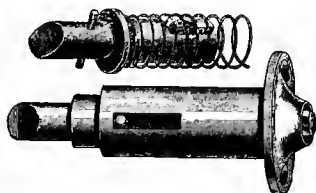
Figs. 4029-4030. SEAT-BACK ARM-LOCK, BOLT AND SPRING.
